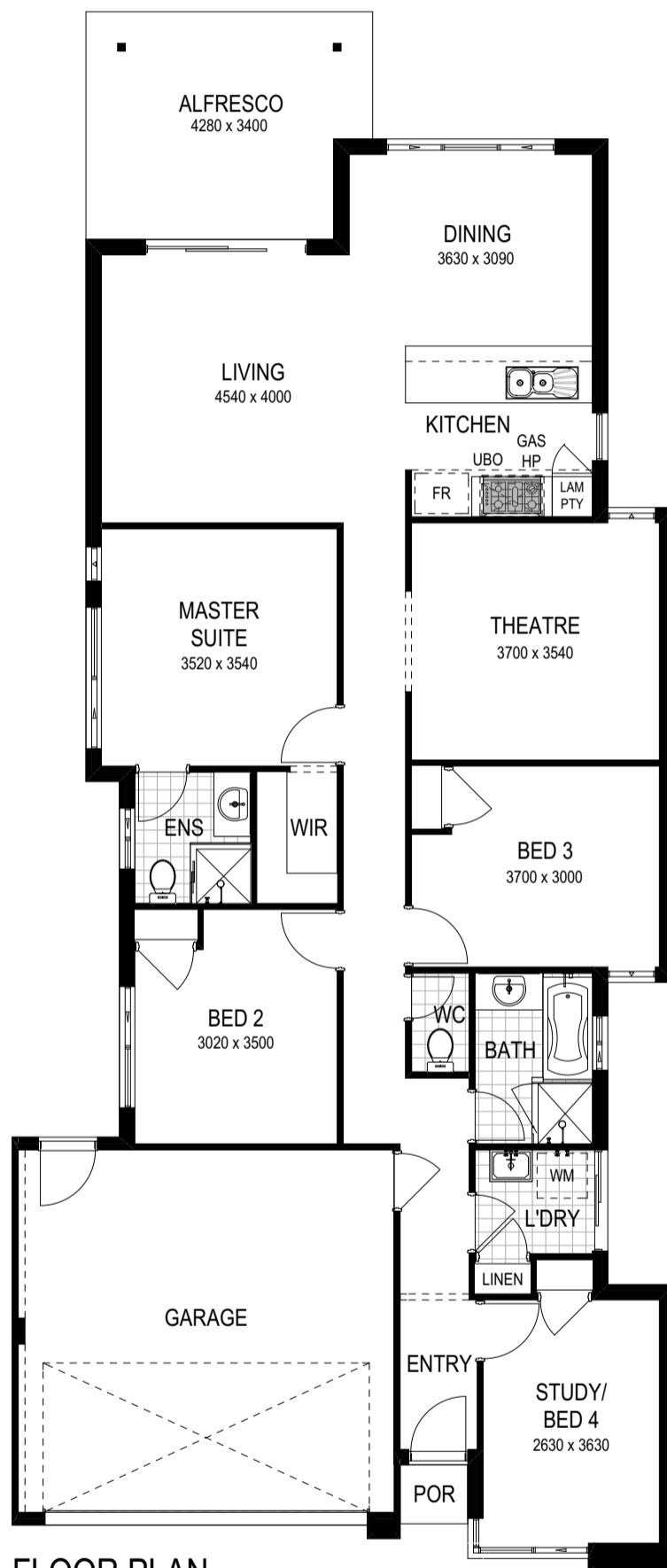
FLOOR PLAN
