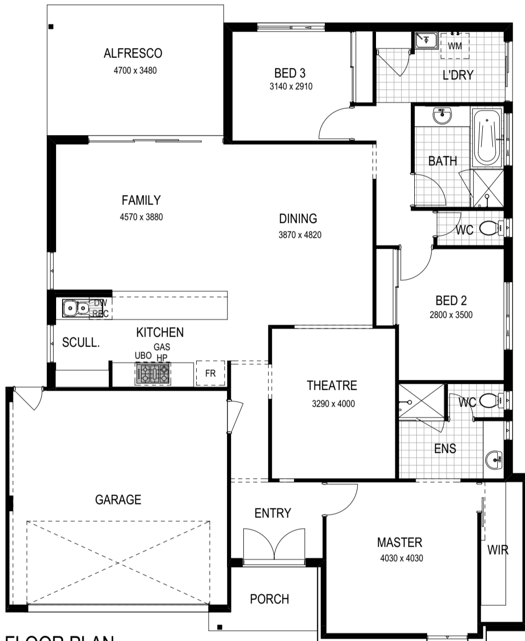
FLOOR PLAN 1:100
