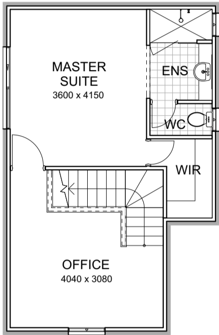
UPPER FLOOR PLAN 1:100
