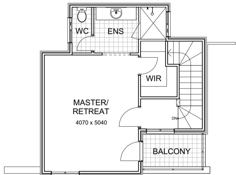
UPPER FLOOR PLAN 1:100
