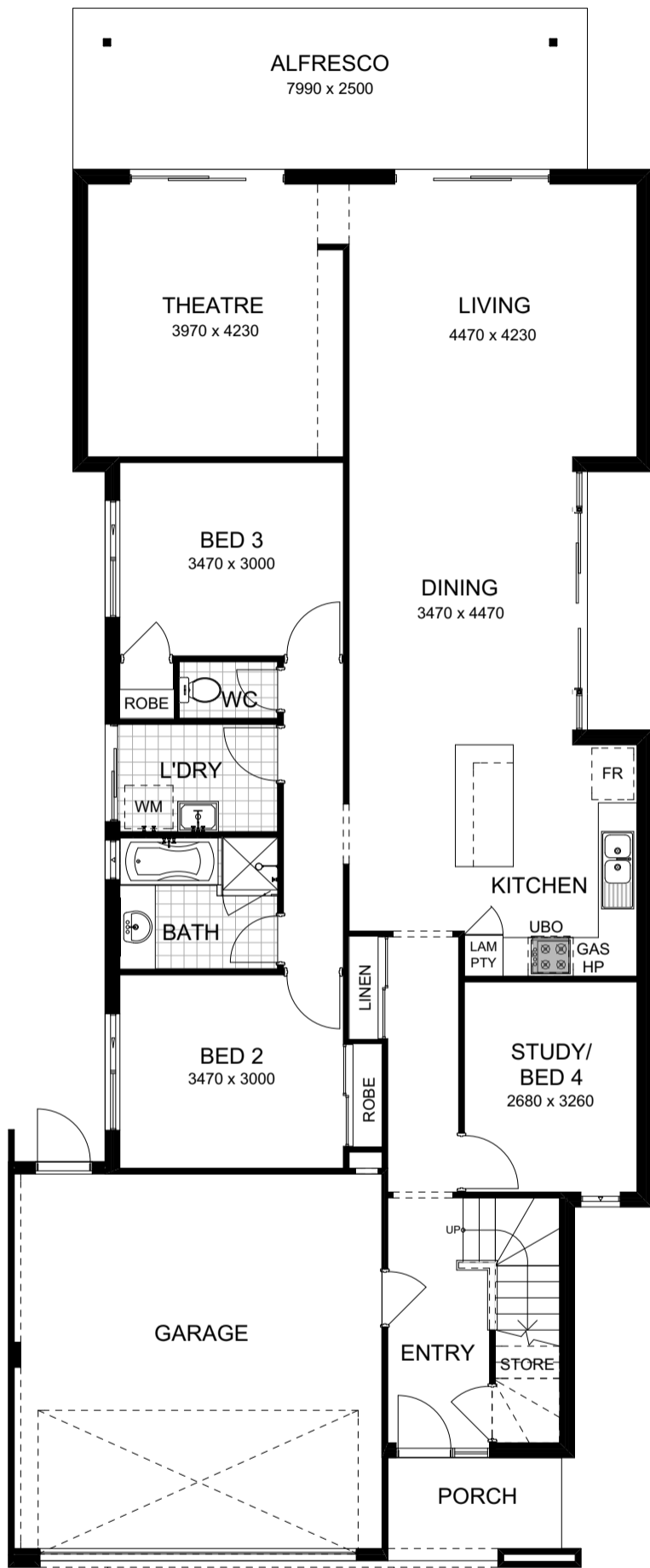
GROUND FLOOR PLAN 1:100
