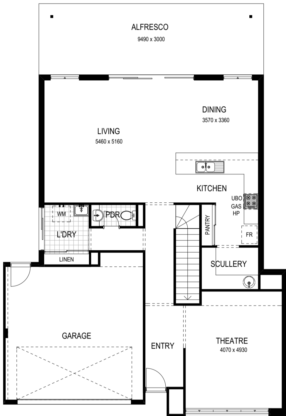
FLOOR PLAN 1:100
